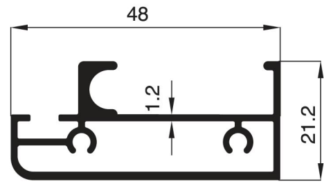
2108 - 0.625 Kg/m
