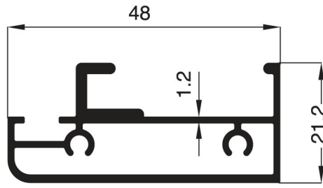
1841 - 0.640 Kg/m
