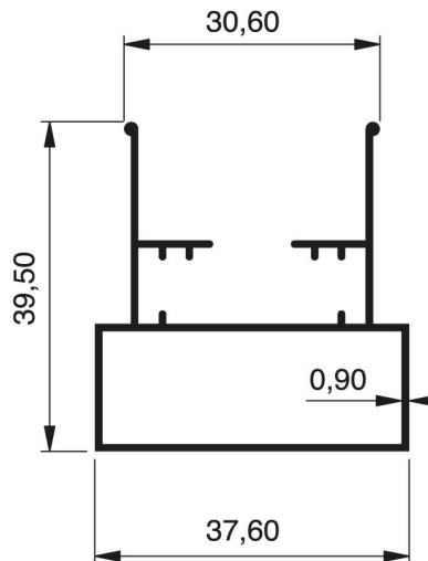
1958 - 0.448 Kg/m
