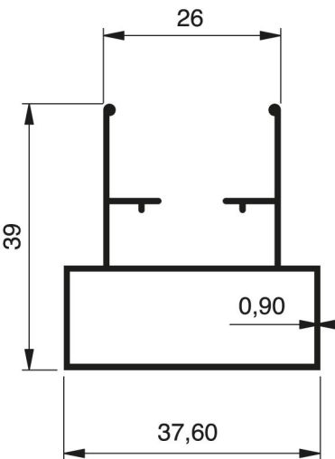
1957 - 0.418 Kg/m
