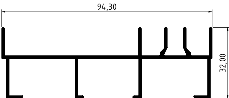
6896 - 0.879 Kg/m
