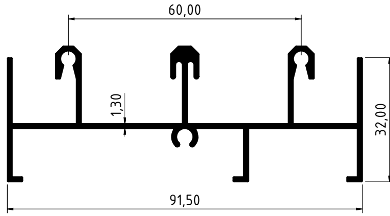
6894 - 1.052 Kg/m
