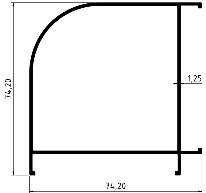
4842 - 0.954 Kg/m
