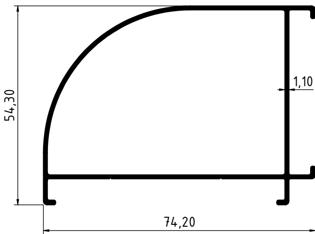
4843 - 0.735 Kg/m
