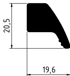
4072 - 0.551 Kg/m
