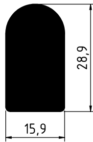
2931 - 1.171 Kg/m
