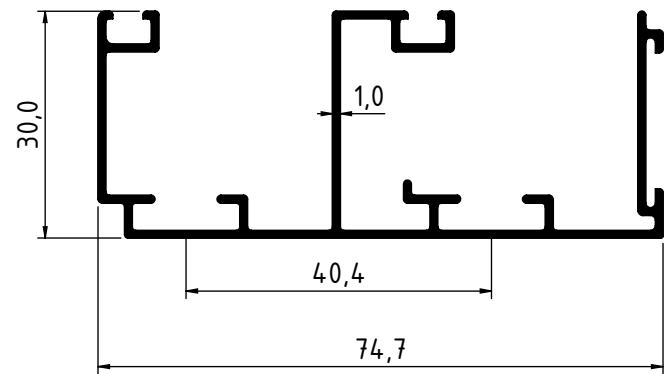
1983 - 0.660 Kg/m
