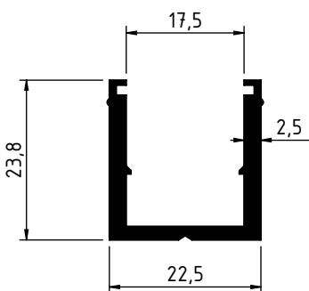
3134 - 0.410 Kg/m
