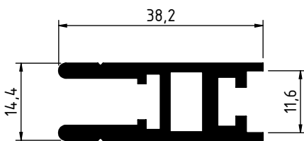
2180 - 0.631 Kg/m
