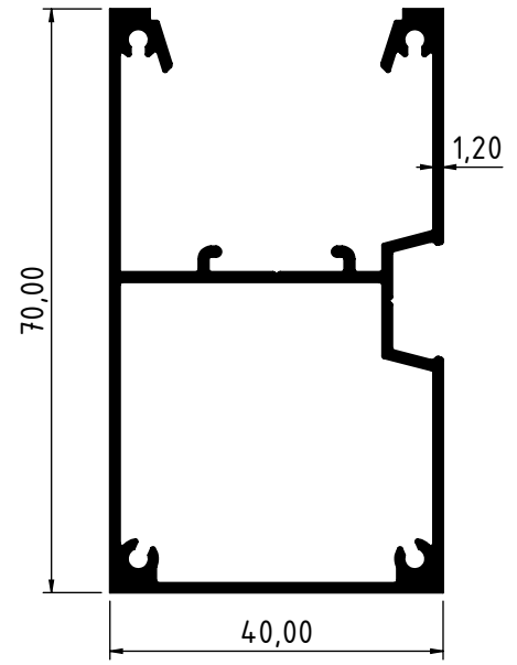
3993 - 0.944 Kg/m
