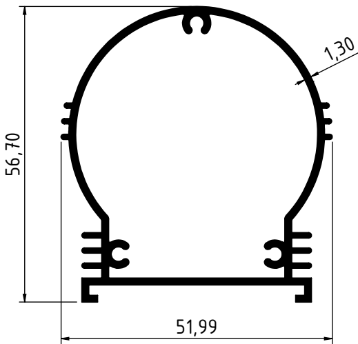
1967 - 0.837 Kg/m
