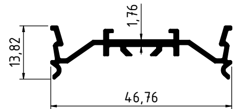
2845 - 0.339 Kg/m
