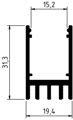
2825 - 0.418 Kg/m
