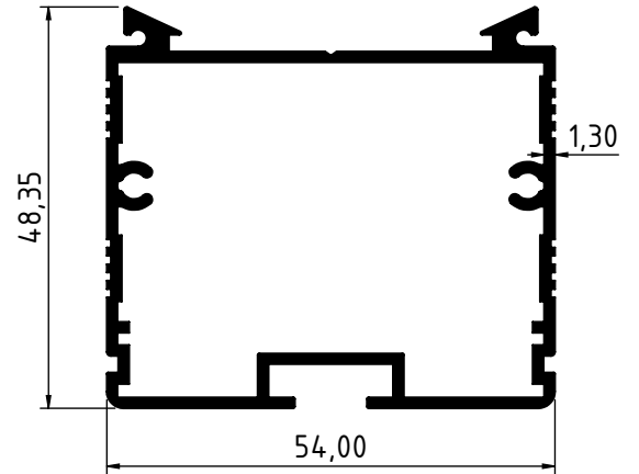
2693 - 0.950 Kg/m
