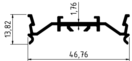
2845 - 0.339 Kg/m
