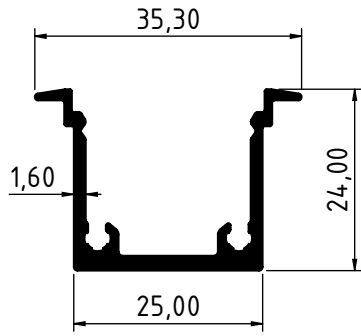
4255 - 0.390 Kg/m
