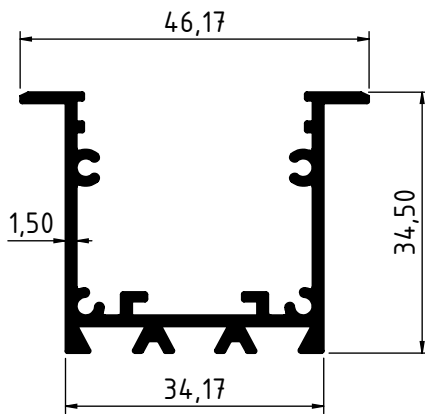
2972 - 0.561 Kg/m
