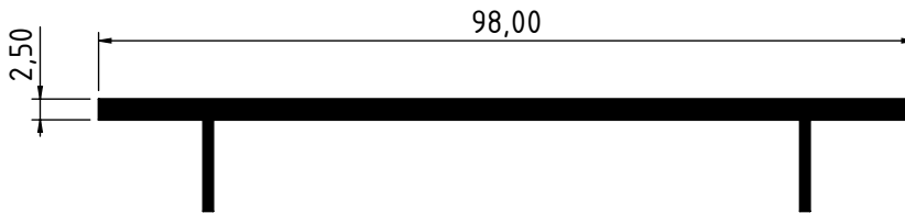
1955 - 0.735 Kg/m
