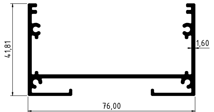
4059 - 0.998 Kg/m
