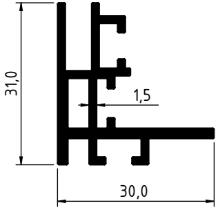
2950 - 0.555 Kg/m
