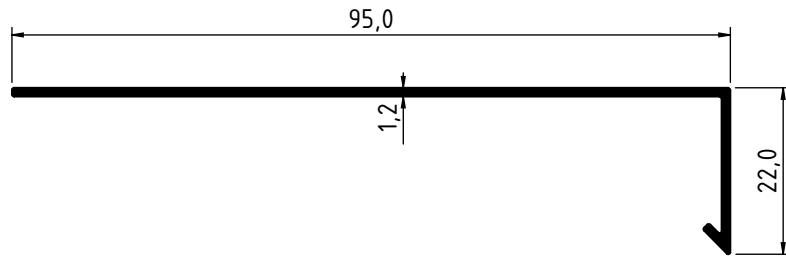
1954 - 0.370 Kg/m
