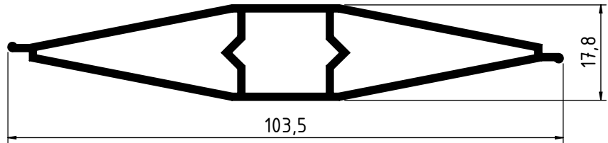
1818 - 0.841 Kg/m
