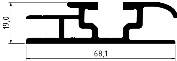
1855 - 1.085 Kg/m
