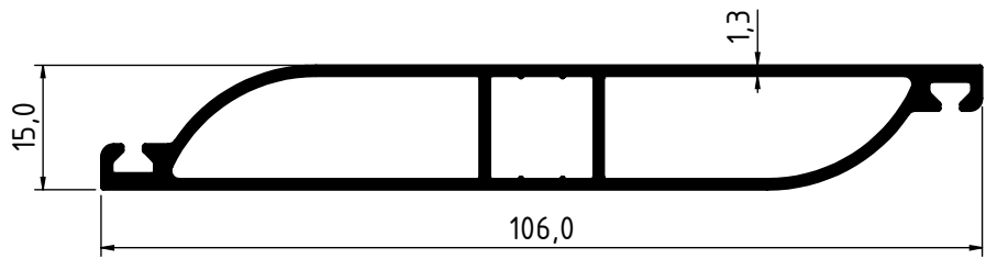
1818 - 0.841 Kg/m
