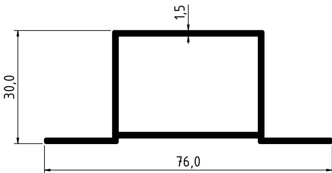
2550 - 0.692 Kg/m
