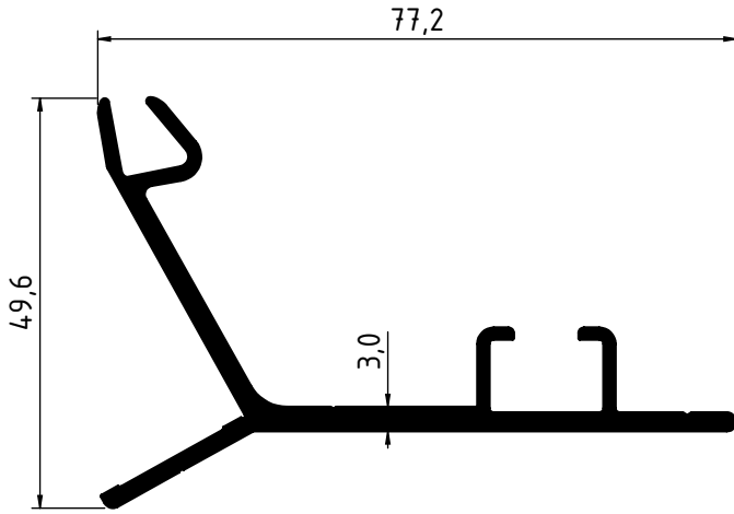
1854 - 0.963 Kg/m
