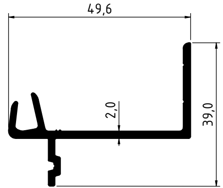
1858 - 0.559 Kg/m
