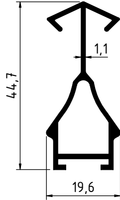
1915 - 0.385 Kg/m
