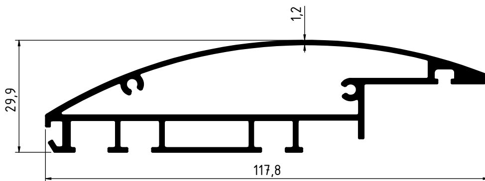
2822 - 1.371 Kg/m
