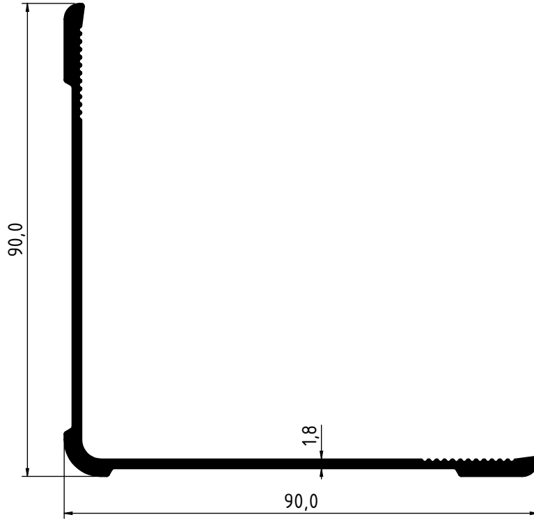
4442 - 0.996 Kg/m
